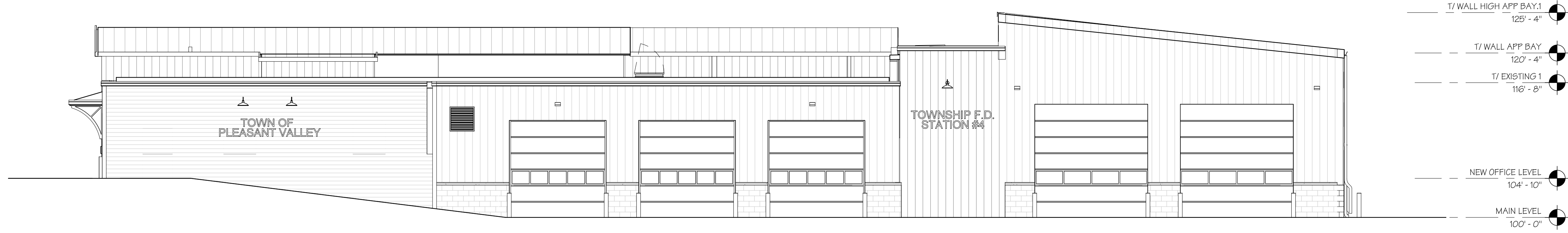
1 EAST ELEVATION 1/8" = 1'-0"
